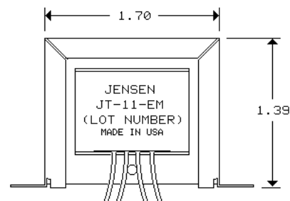
#24 AWG (7x32) UL STYLE 1061 COLOR CODED WIRE LEADS, 8" MINIMUM LENGTH
