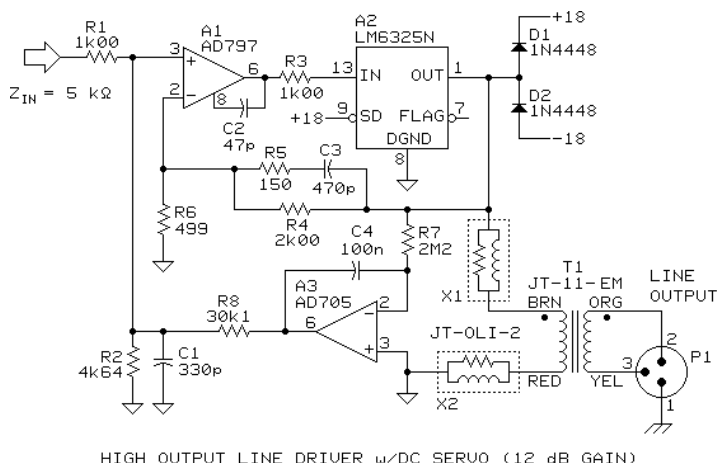
HIGH OUTPUT LINE DRIVER w/DC SERVO (12 dB GAIN)
